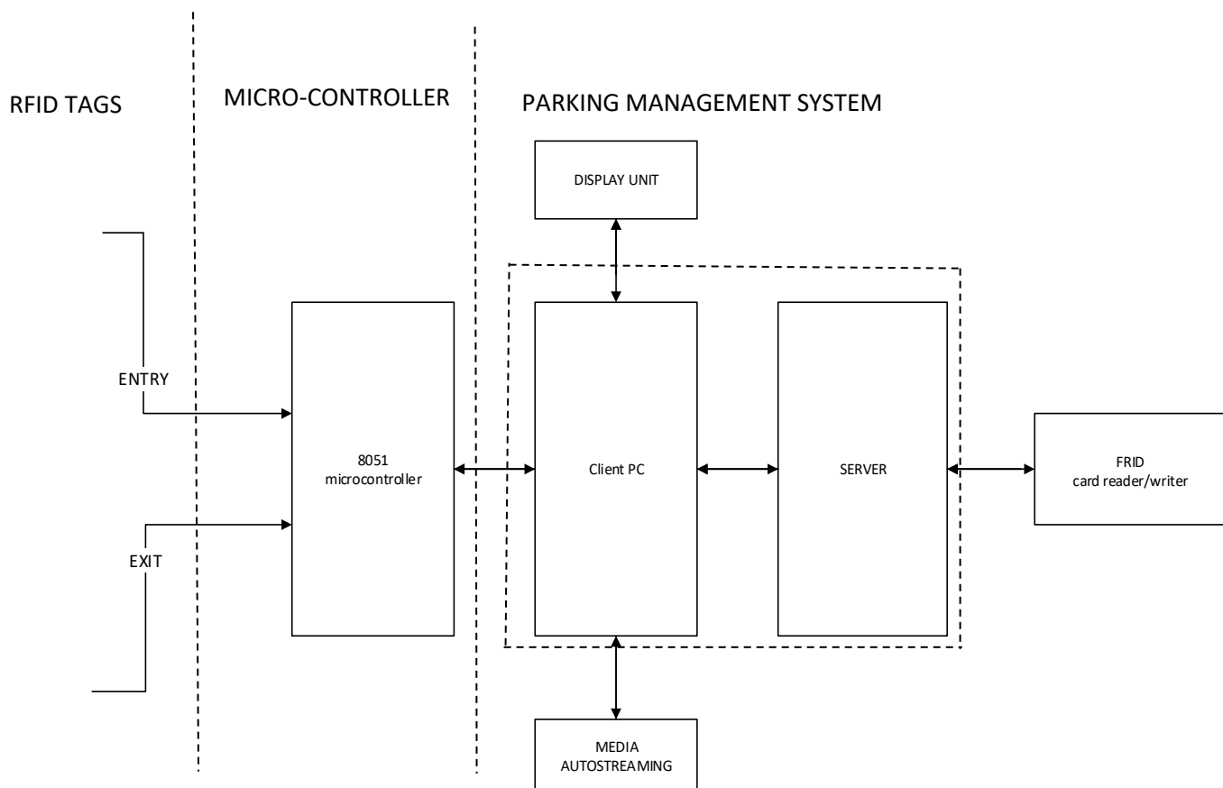
Fig 1: Framework of RFID With Media Intergration
